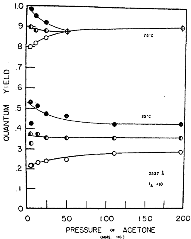
Fig. 2. Effect of pressure and temperature on quantum yields at 2537 Å. (Herr and Noyes (36).)
