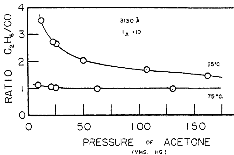
FIG. 5. Effect of pressure and temperature on C 2 H 6 /CO ratio at 3130 Å. (Herr and Noyes (36).)
