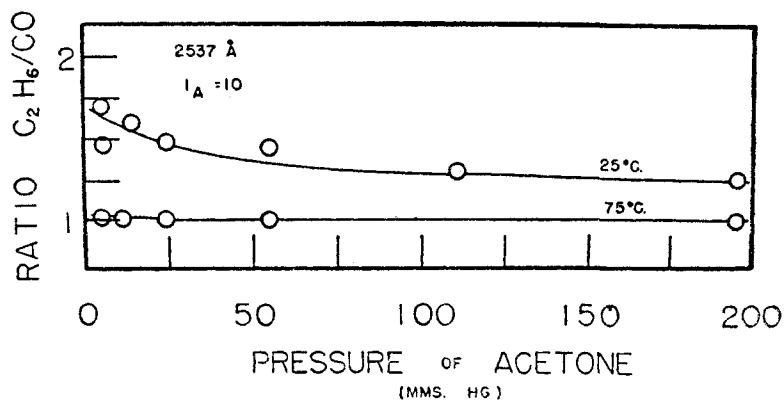
FIG. 6. Effect of pressure and temperature on C 2 H 6 /CO ratio at 2537 Å. (Herr and Noyes (36).)
